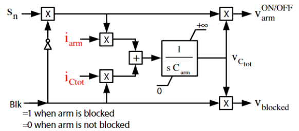
Fig. 3. Equivalent capacitor voltage calculation.
